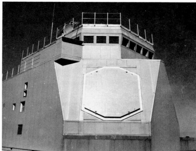
Fig. 3 Modern phased-array radar , the AN/SPY-1A, is used in air-defense system on Navy ships, four antenna faces per ship. This face is on the developmental site at Missile and Surface Radar, Moorestown.
