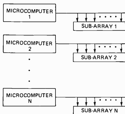
a. Multicomputer beam steering control.
