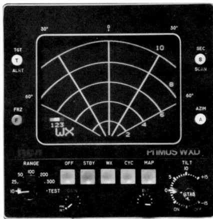
Fig. 7 High-resolution dot pattern for range azimuth markers is difficult to produce on a 525-line tv raster. Special LSI circuit makes the dots appear as smooth lines.
