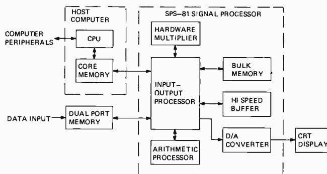
Fig. 2 Signal-processing system. A typical application architecture involving host computer control, display, and data/signal processing flow from input to computational output deposited in the host computer memory.
