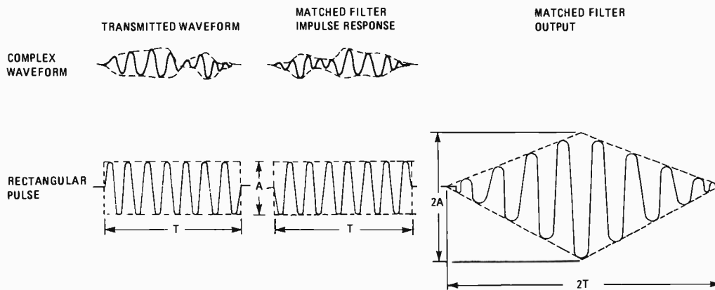
Fig. 7 Matched filtering between transmitted waveform and receiver output produces the maximum S/N. It does not preserve the shape of the original transmitted pulse as seen with the example of the rectangular pulse.
