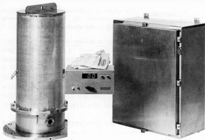
Fig. 3 System has three major components—microwave electronics/antenna enclosure (left) and signal-processing enclosure (right), which are installed on the furnace top, and display enclosure, which goes in furnace control room.
