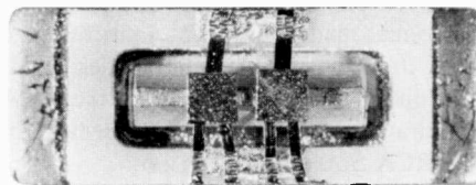
Fig. 2 "Flipped" device mounted on a gold-plated copper carrier. This technique provides good heatsinking and low source inductance.
