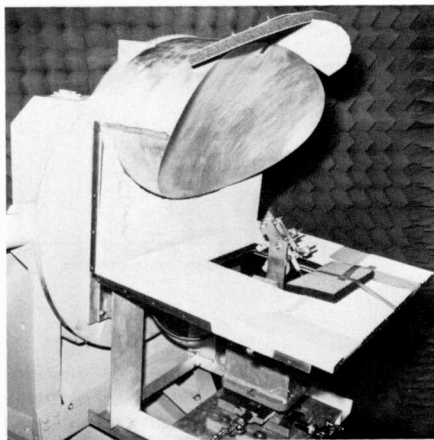
Fig. 6 One-tenth scale model verified low-sidelobe responses predicted by computer simulation. Operating frequency covers 31 GHz to 36 GHz. Test feed horns were designed to provide either horizontal or vertical linear polarization.
