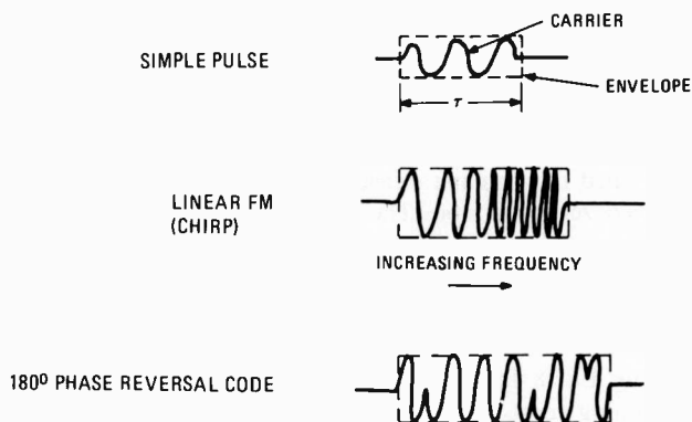
Fig. 8 Typical radar waveforms. Simple pulse is formed by rectangular modulation of the rf carrier. "Chirp" waveform, used to achieve high range resolution at moderate transmission power, is actually a long pulse generated by delaying different frequency components of a short pulse. Phase-reversal codes are used to obtain pulse compression for low as well as high time-bandwidth products.
