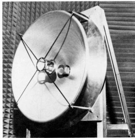
Fig. 10 A new wideband multimode monopulse feed for a small Cassegrain antenna. The new mode-generating technique has doubled bandwidth capabilities.
