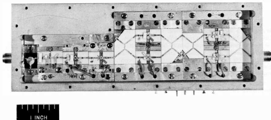
Fig. 4 Experimental amplifier was produced in a microwave integrated circuit format. Note the modular approach taken and compare the modules with the blocks of Fig. 3.
