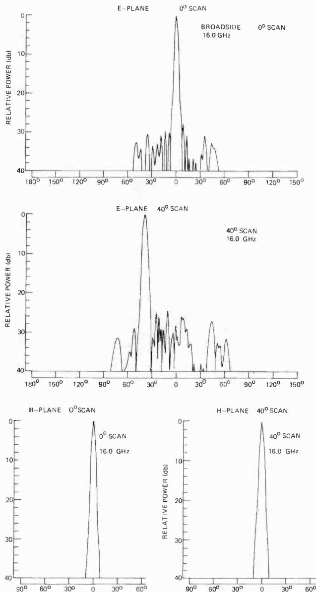
Fig. 13 E-(scan plane) and H-plane patterns of the low-sidelobe phased array with dual-mode sectoral horn power divider.
